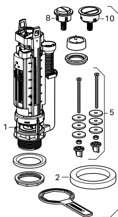
Flushing Valve Type 290 Dual-flush
