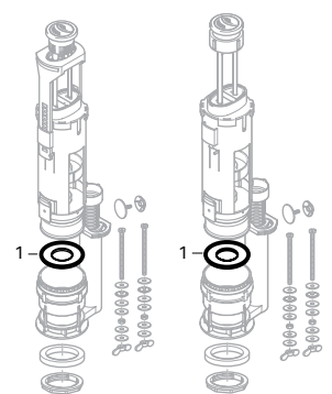
Flushing Valve Type 250† Dual-flush
